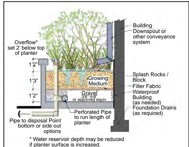
Figure 7.44 Schematic of Flow-through Planter Box
