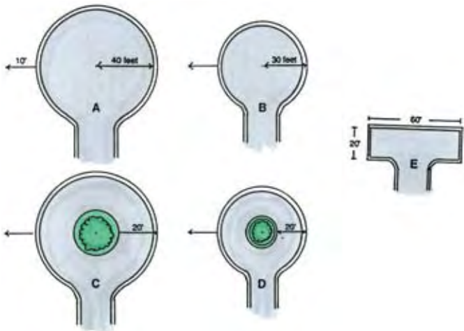
Figure 6.5 Five cul-de-sac options
