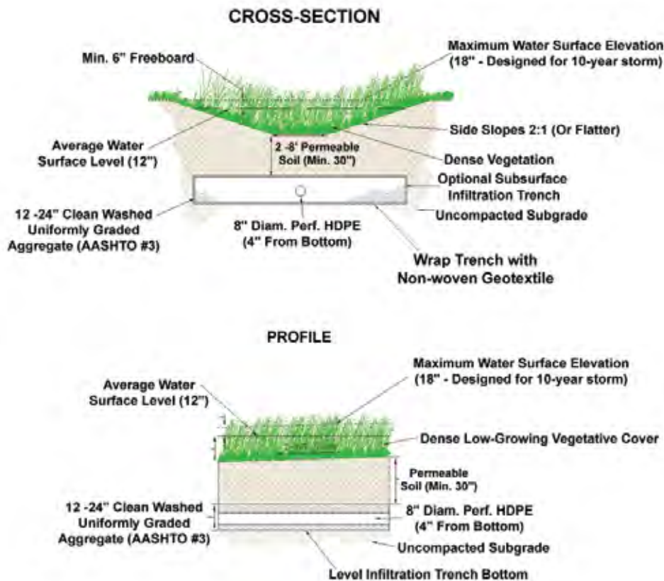
Schematics of Vegetated Swale with an underlying aggregate layer
