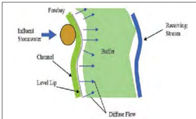
Level spreader located between a sediment forebay and a buffer
