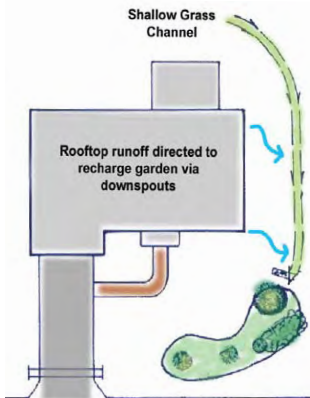
Single-family residential lot drainage schematic
