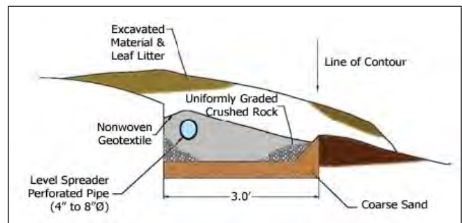
Level spreader with geotextile surrounding the aggregate helping to create a sloped area.
