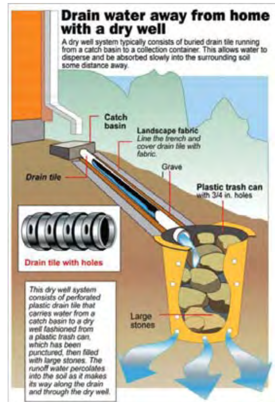
Residential dry well
